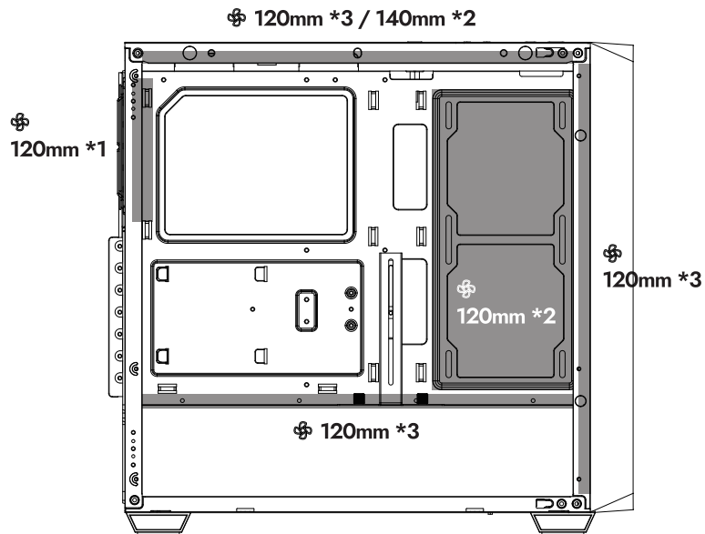
"FAN SUPPORT"
