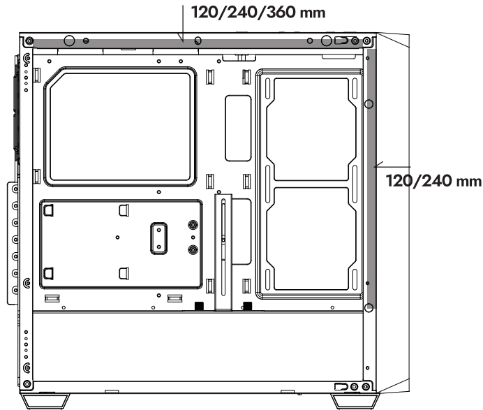
"RADIATOR SUPPORT"
