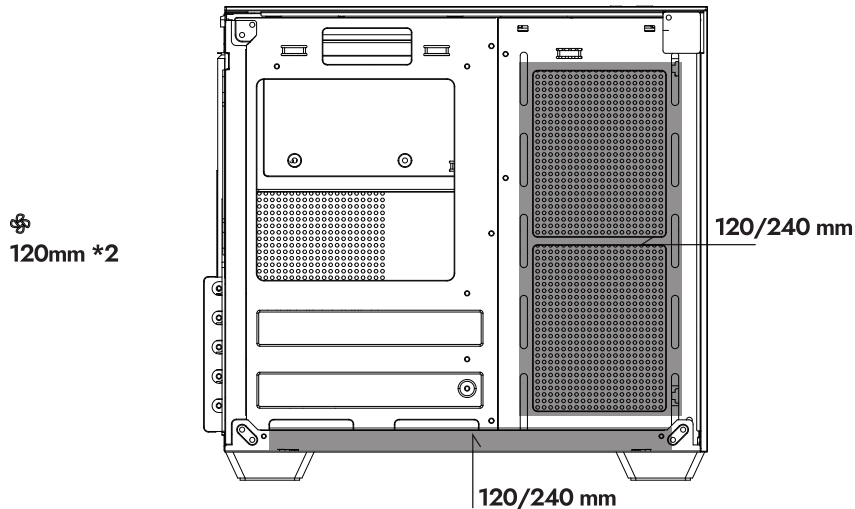
“RADIATOR SUPPORT”
