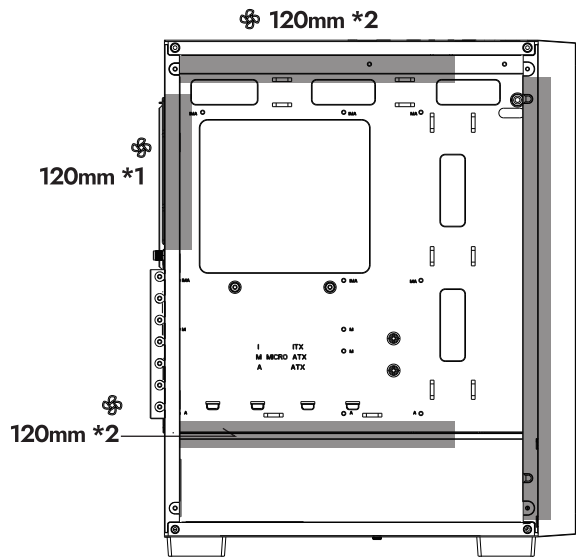
"FAN SUPPORT"
