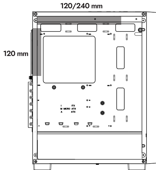
"RADIATOR SUPPORT"
