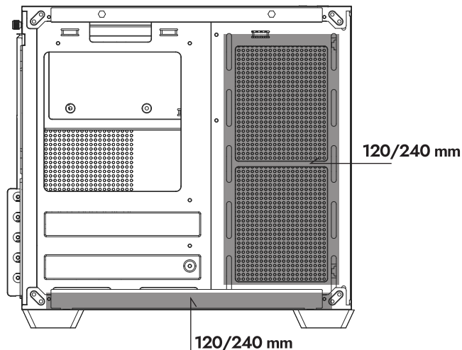
"RADIATOR SUPPORT"
