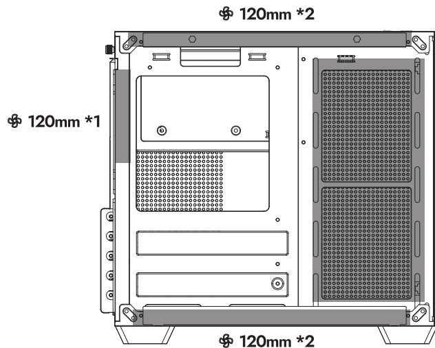
"FAN SUPPORT"
